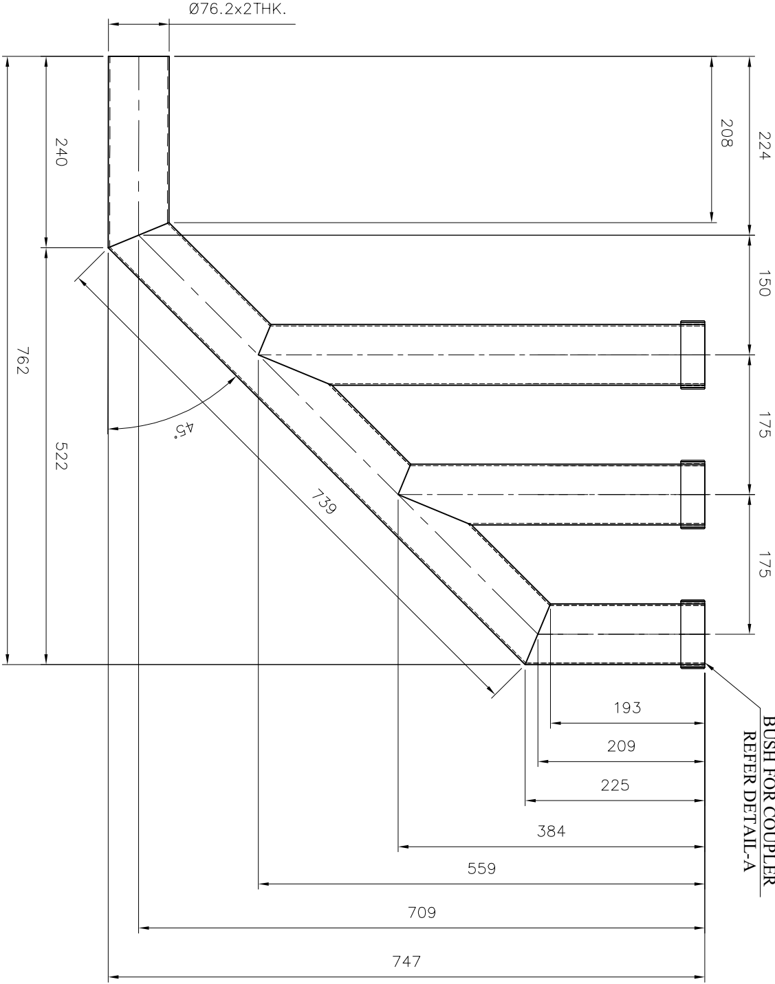
DETAIL OF BRANCH PIPE
